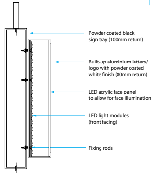
Side elevation detail
