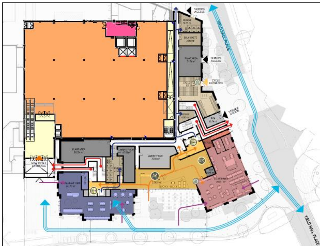
Figure 6.2: Yield Hall Place 1 Entrances and Cycle Parking
