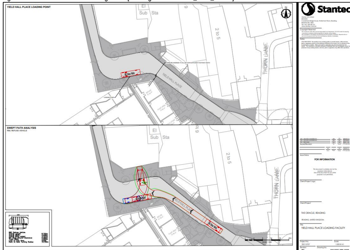
Figure 6.4: Yield Hall Place 1 Servicing Areas [Drawing No.332110757_5500_SK020]
