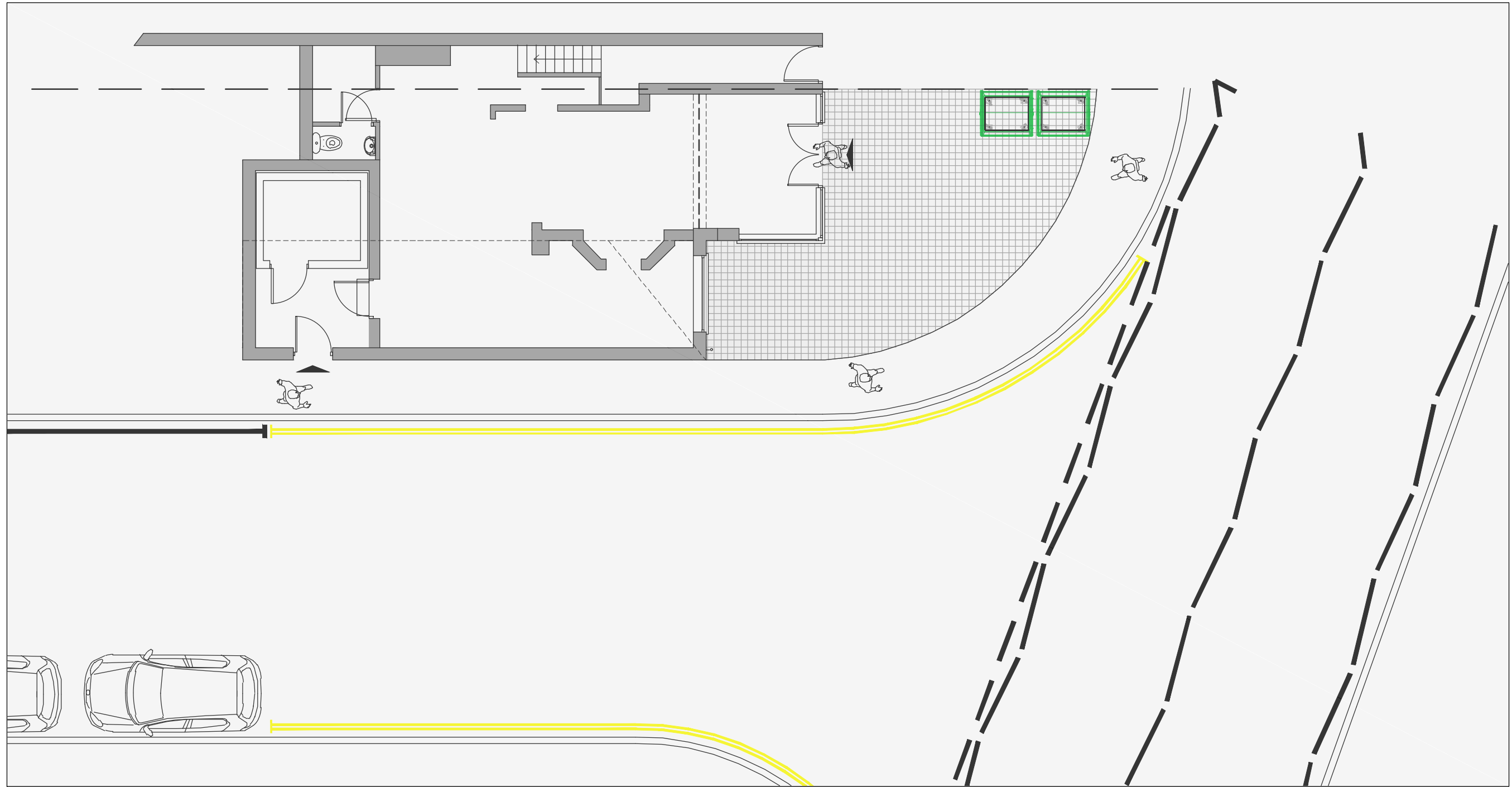
Existing Landscape Plan Scale 1:100
