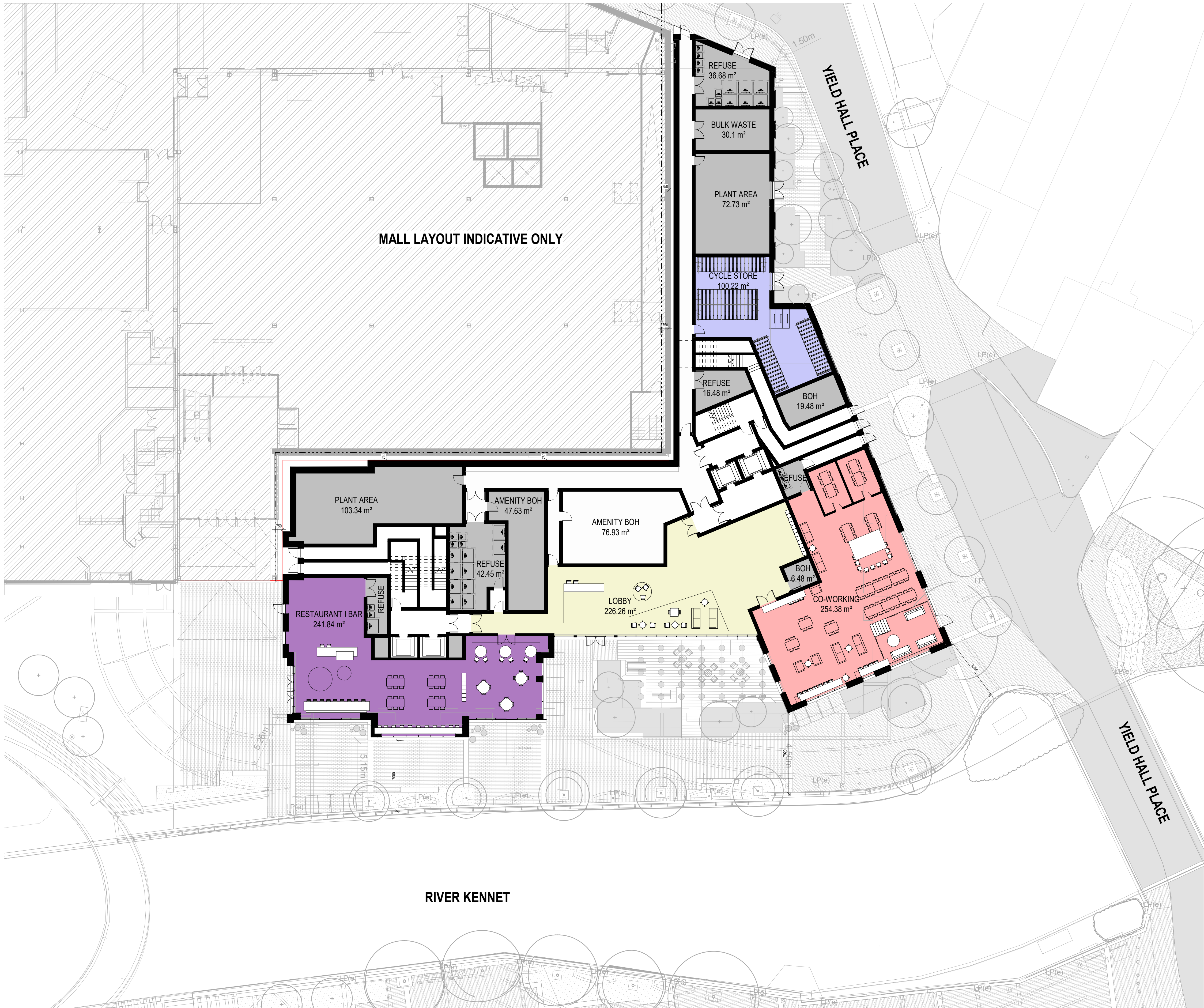
1 GA PLAN - YIELD HALL PLACE 1 - A-B - LEVEL 00 - GF SCALE: 1 : 200
