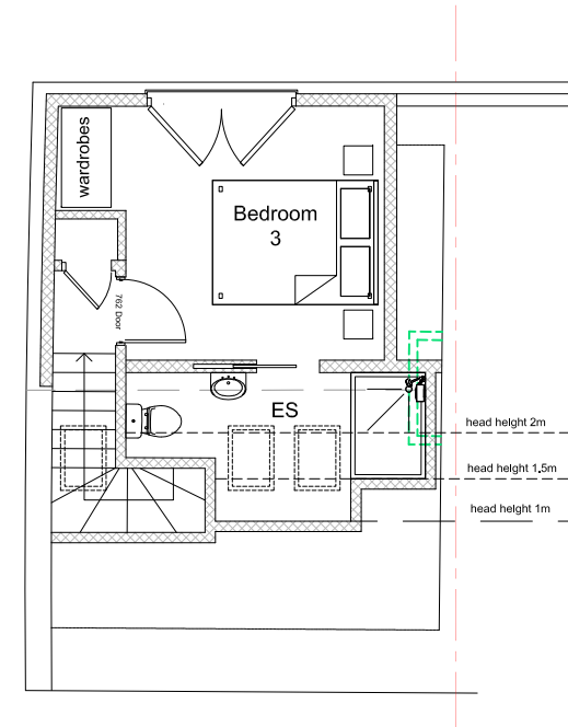
PROPOSED LOFT PLAN
