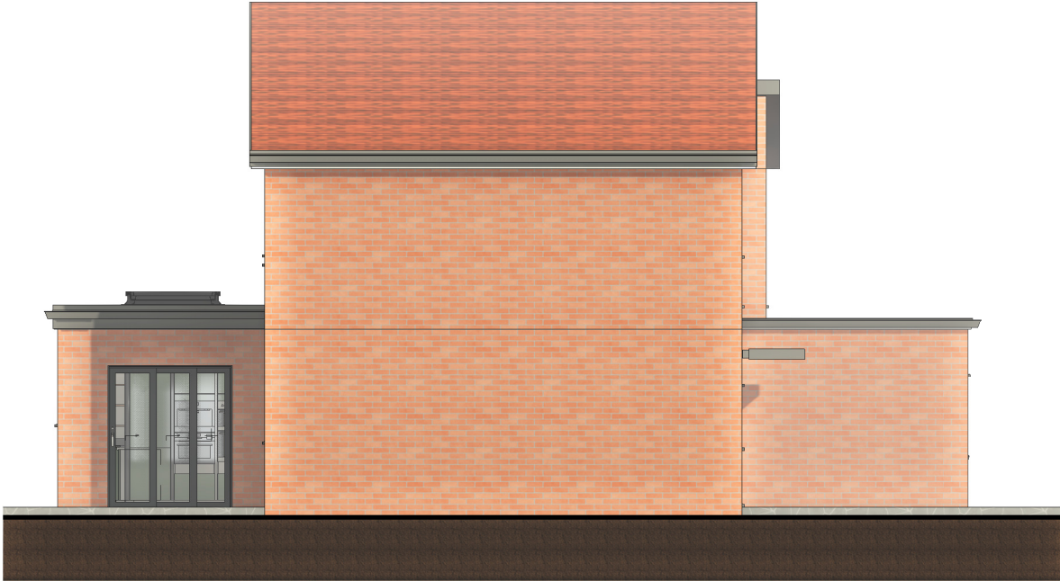
2 East. Coloured 1 : 100
