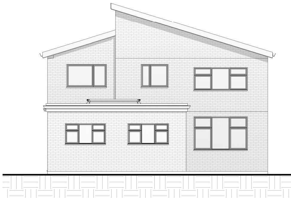
3 South. 1 : 100
