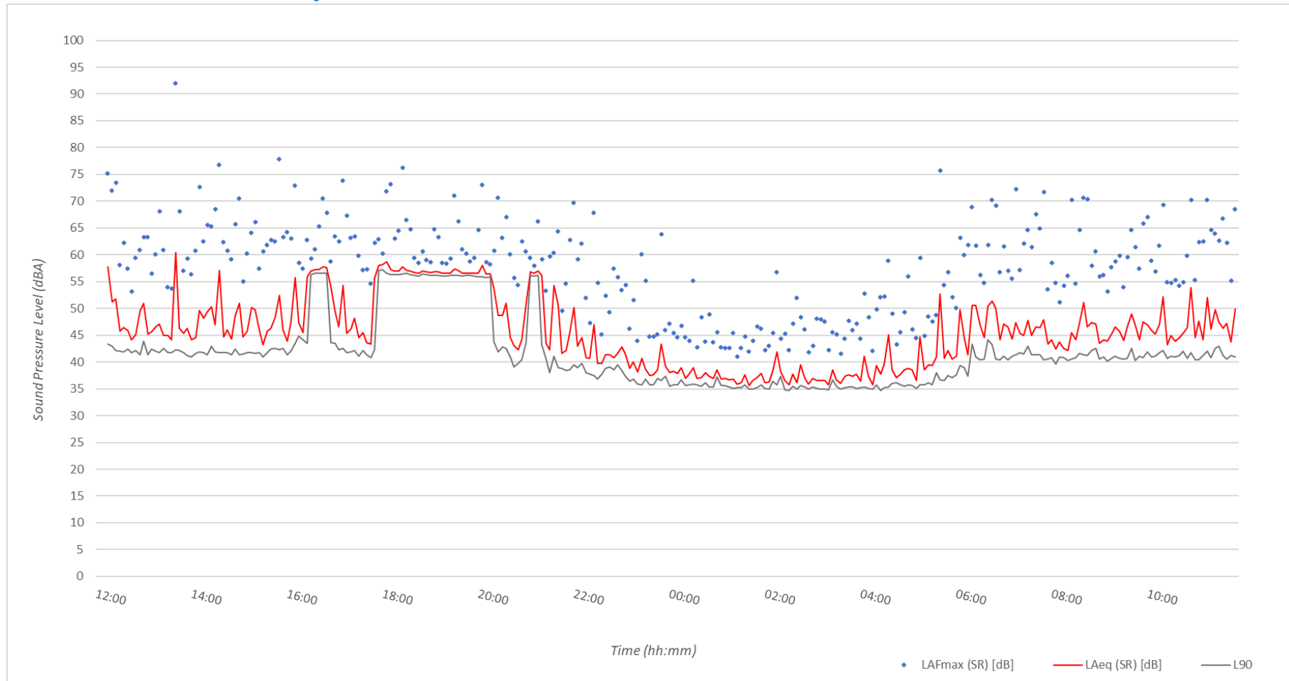
Figure 5: Measured Background Sound Levels Time History (M1): 29 th – 30 th April 2024
