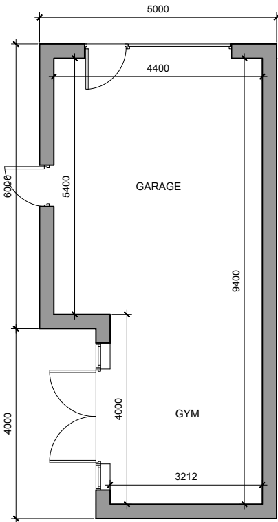
PROPOSED GARAGE PLAN
