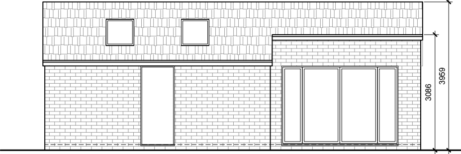
PROPOSED LEFT SIDE ELEVATION
