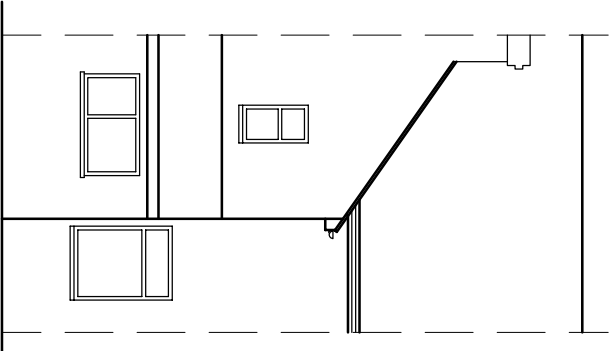
EXISTING REAR ELEVATION
