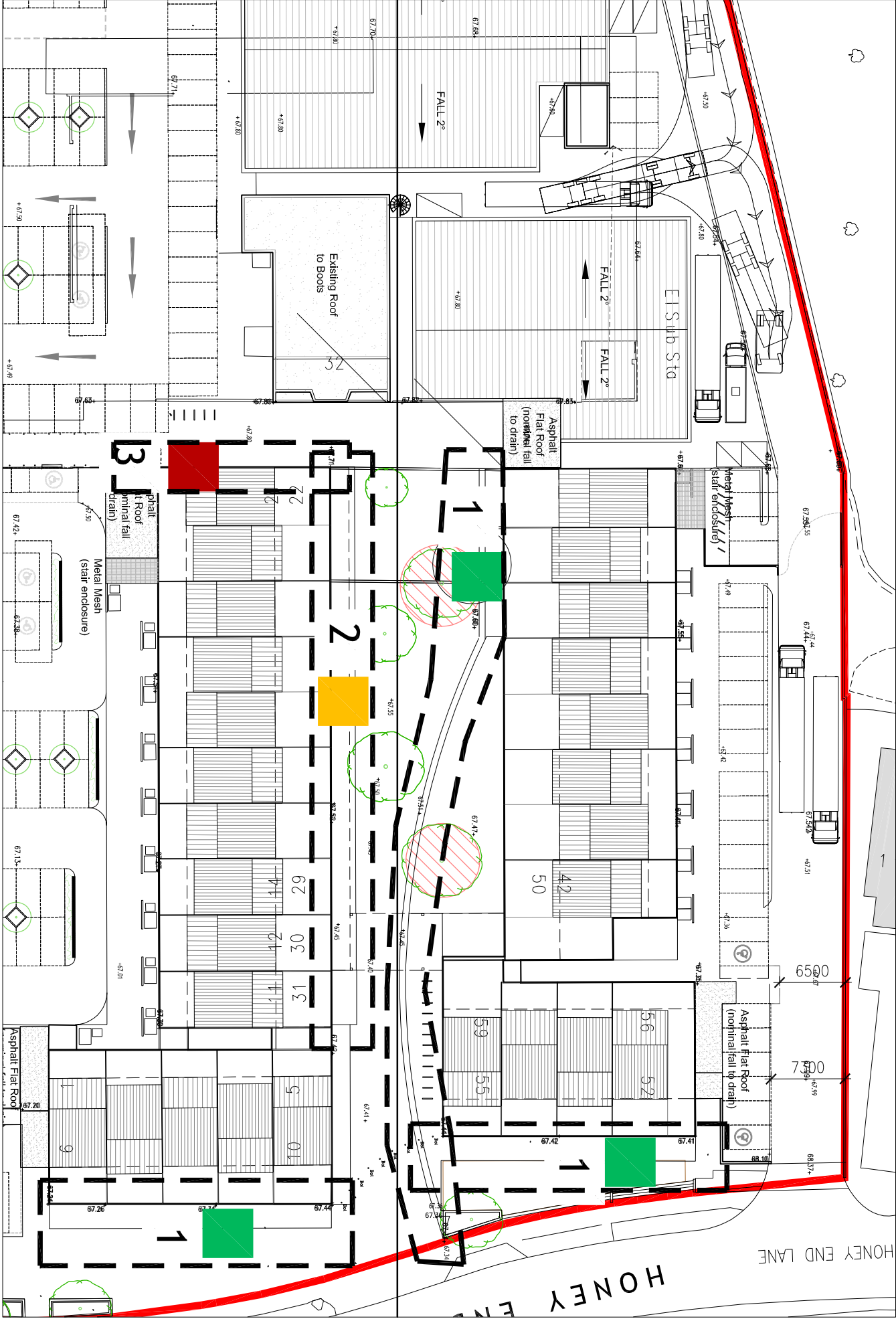
Proposed Canopy Details Part Plan - Scale - 1:500
