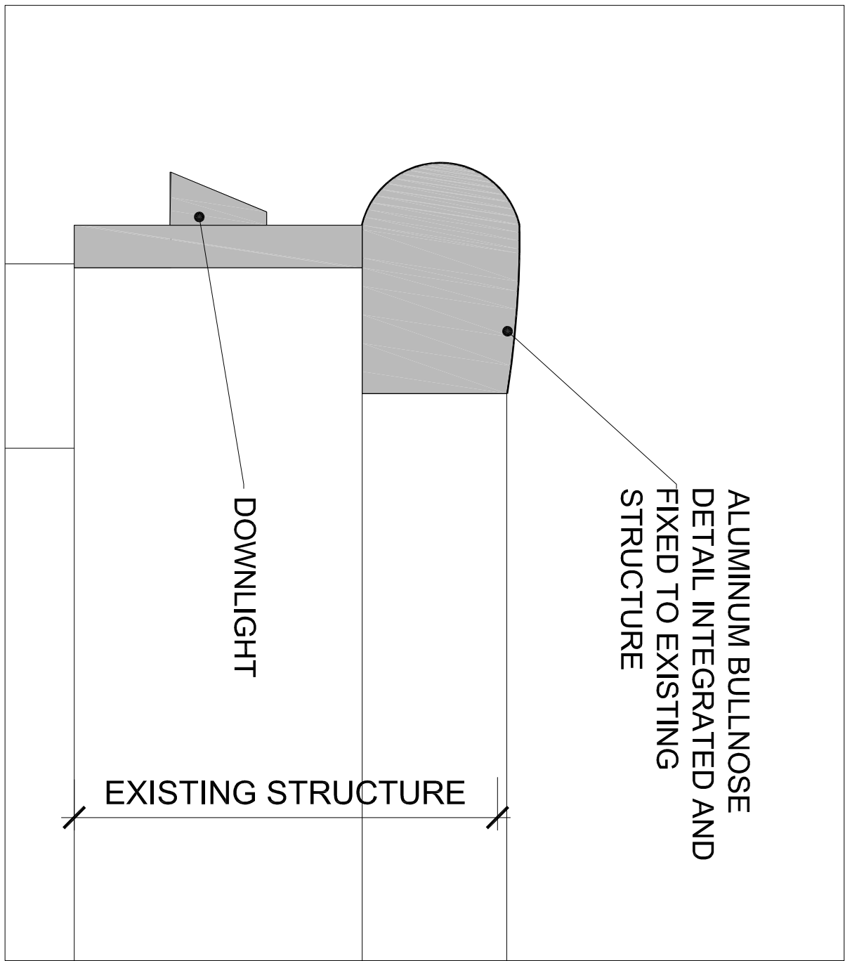
Proposed Canopy Profile '2' - SCALE - 1:10
