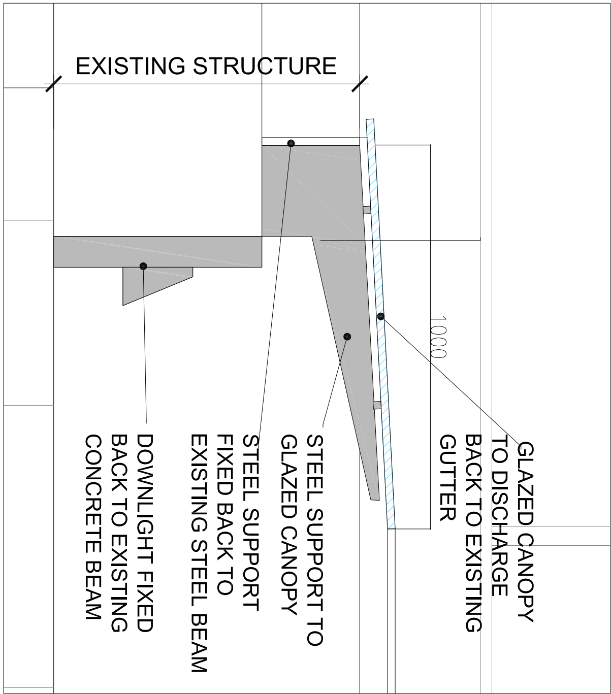
Proposed Canopy Profile '1' - Scale - 1:10
