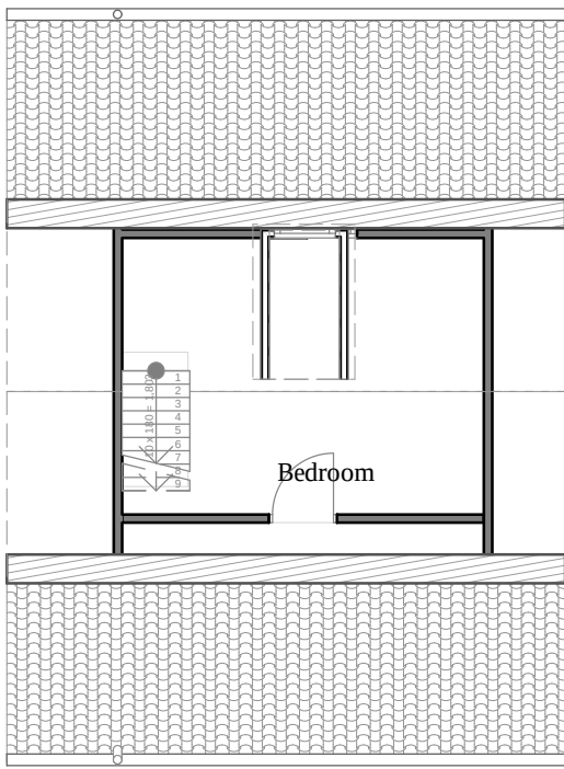
Second Floor Plan 1:100 536 Oxford Road Reading
