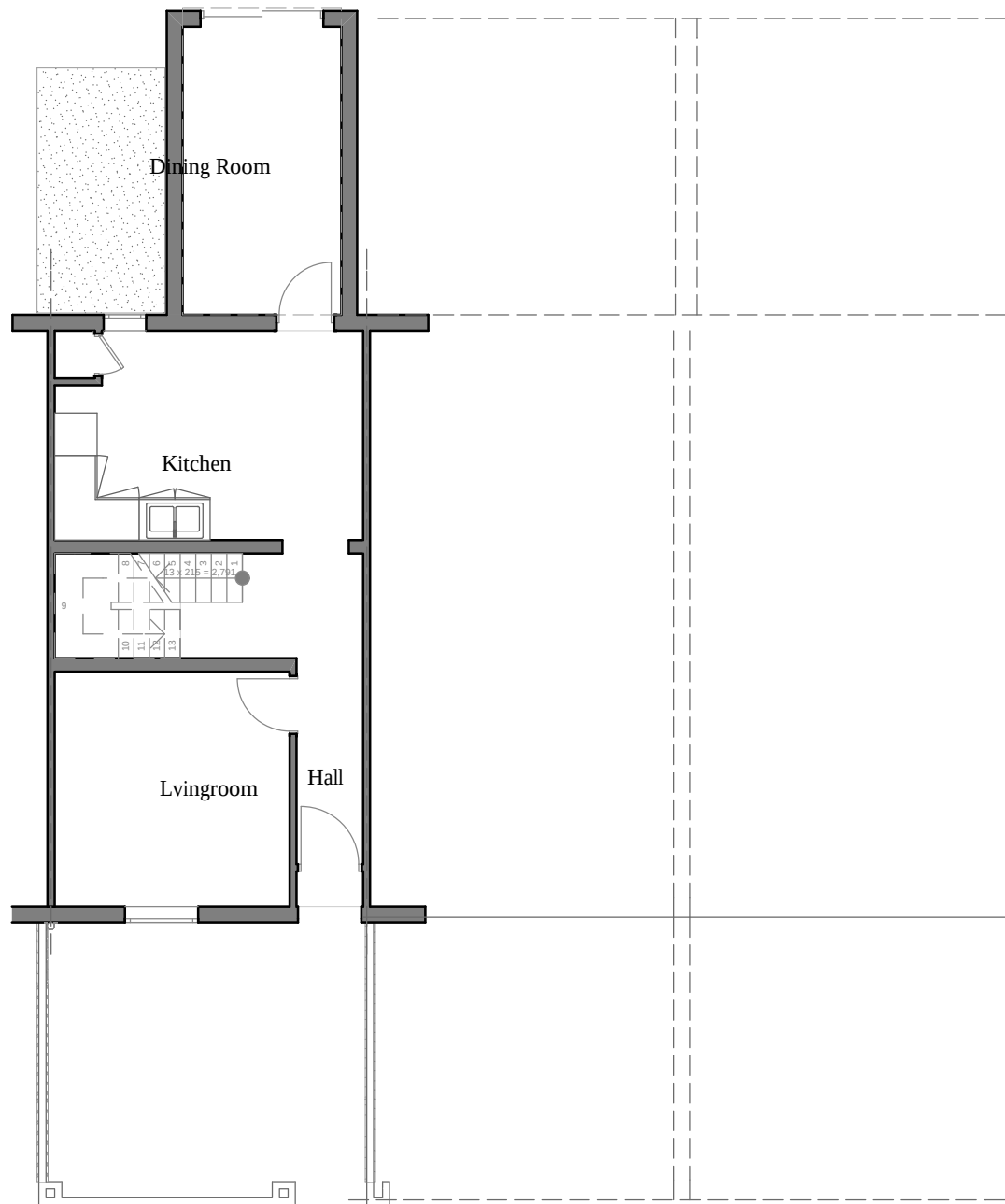
Ground Floor Plan 1:100 536 Oxford Road Reading
