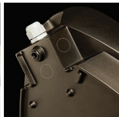
Cable 'Knock Out' points allow simple and flexible installation and through wiring.
