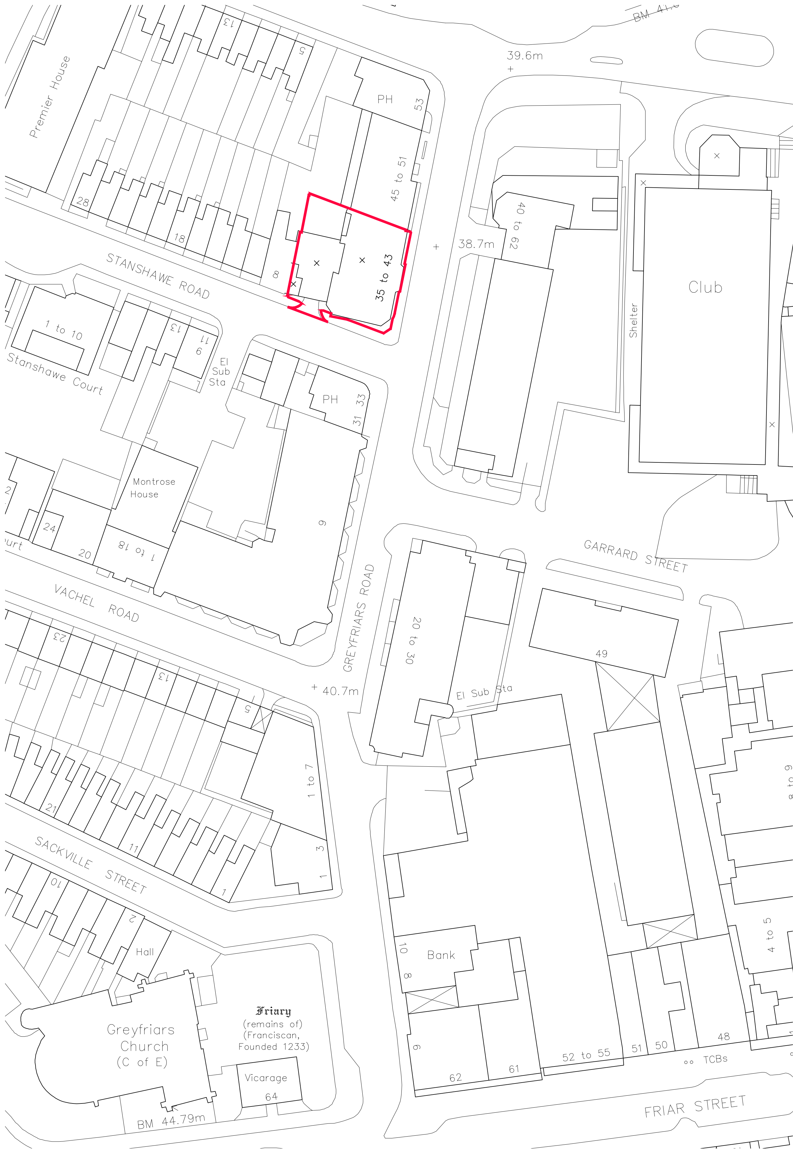
01 Existing Block Plan Scale 1:500@A1, 1:1000@A3
