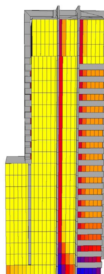
Figure 13: Total APSH - Proposed Scenario
