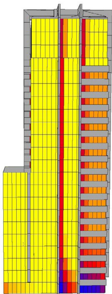
Figure 11: Total APSH - Existing Scenario
