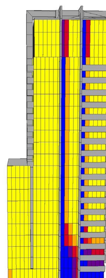
Figure 14: Winter APSH - Proposed Scenario
