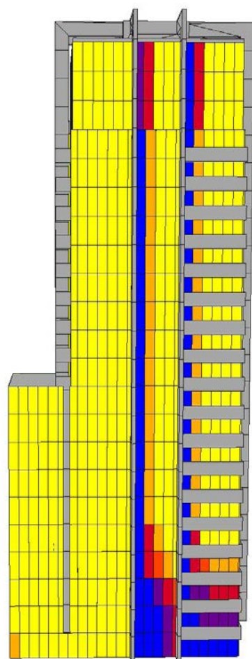
Figure 12: Winter APSH - Existing Scenario
