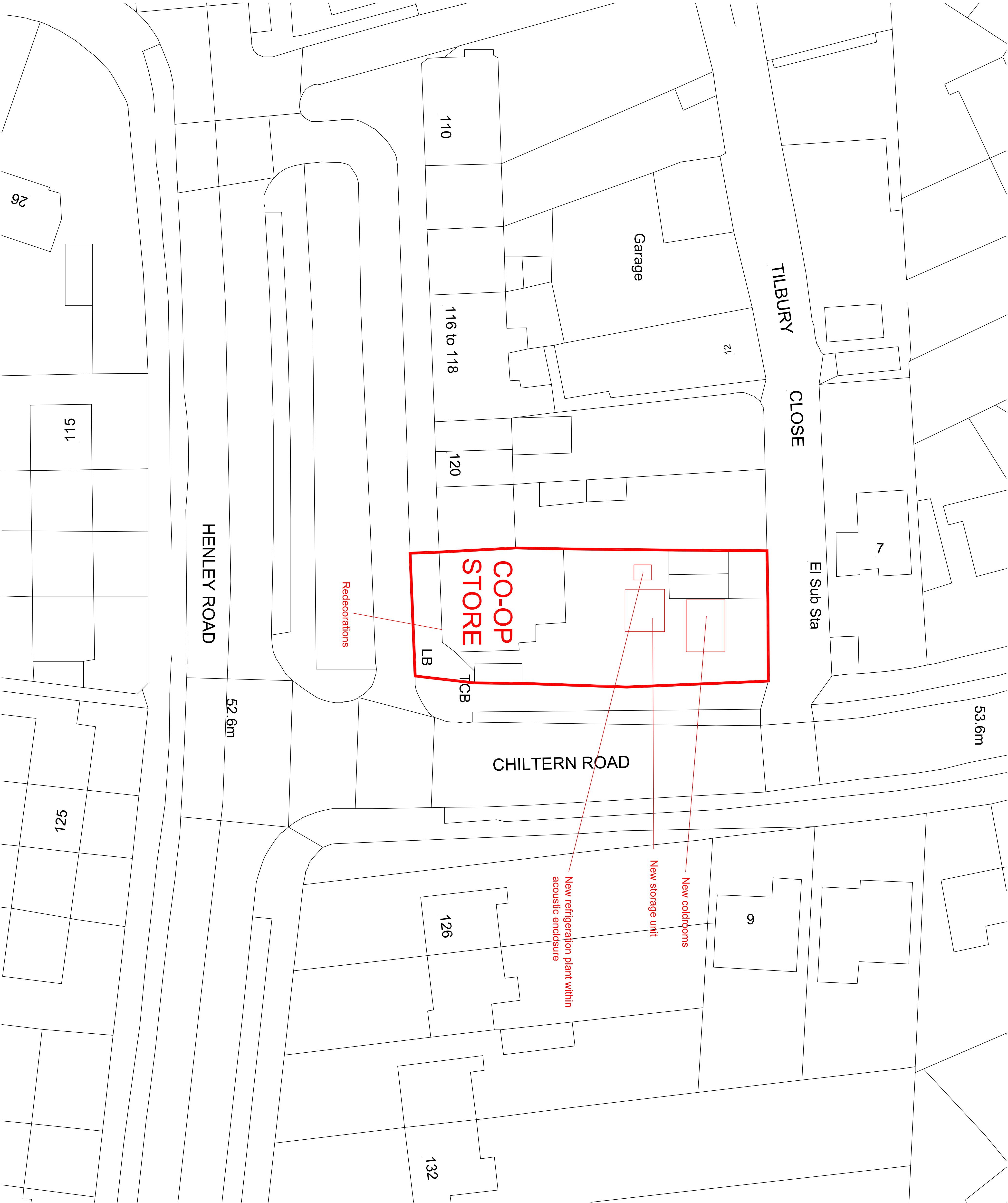
BLOCK PLAN 1:200
