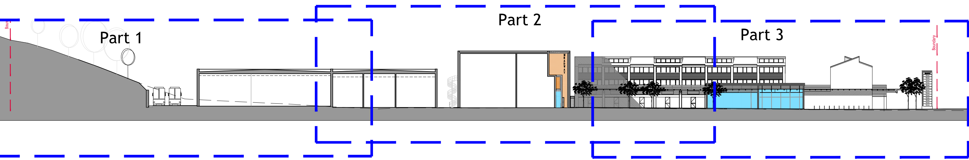
Proposed Section H-H Scale - 1:500
