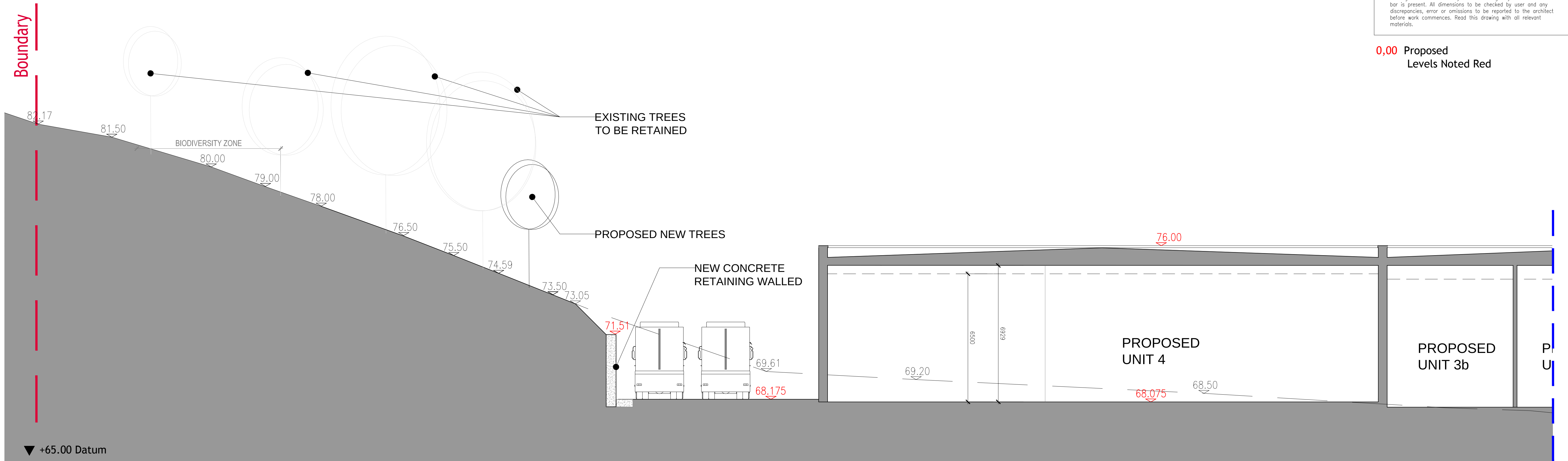
Part 1 - Proposed Section H-H Scale - 1:100
