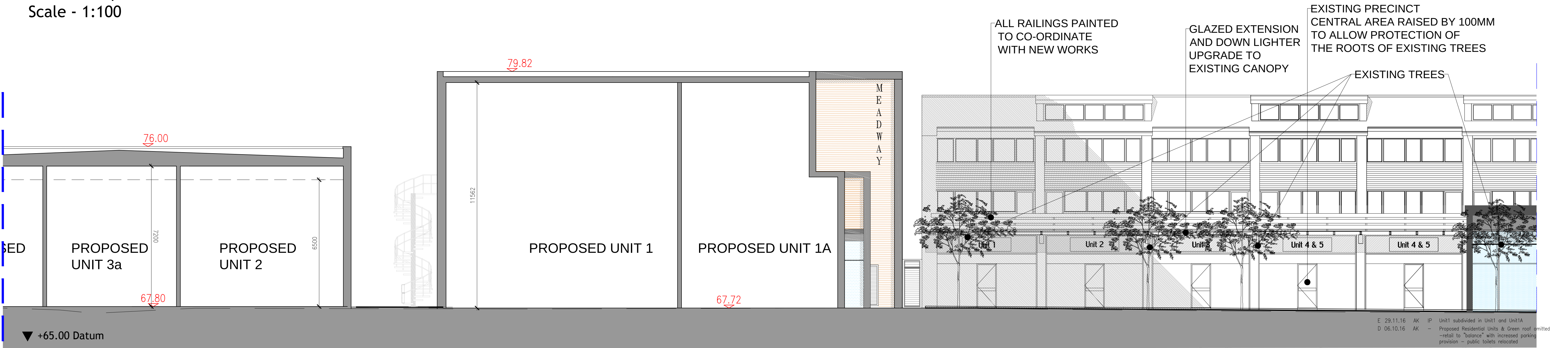
Part 2 - Proposed Section H-H Scale - 1:100
