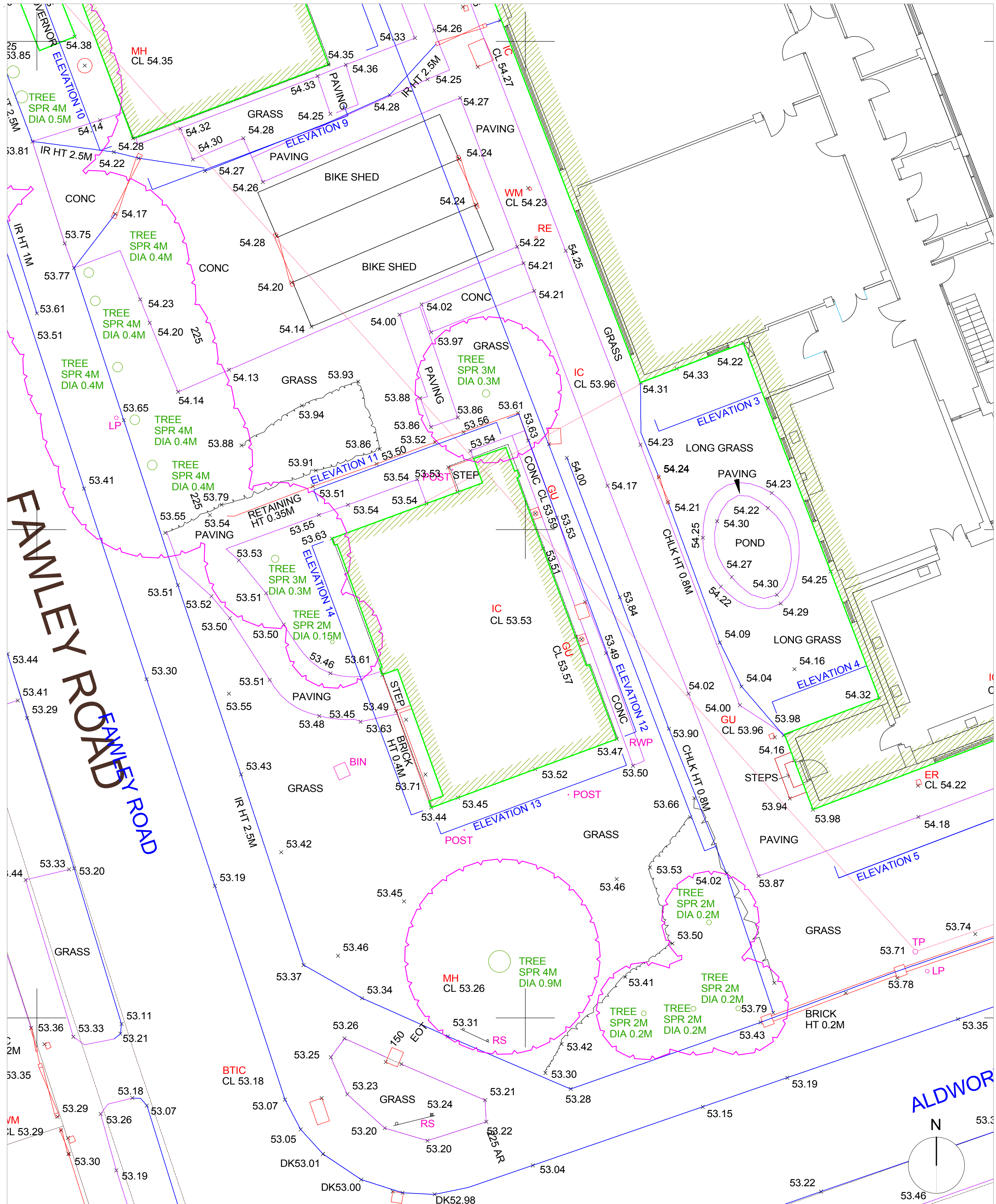
Survey Extract - 1:100 @ A1
