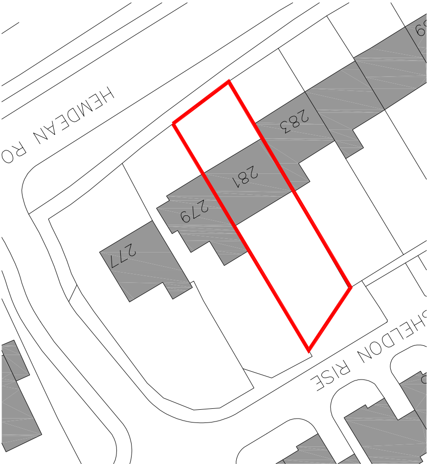
Block Plan Existing 1:500
