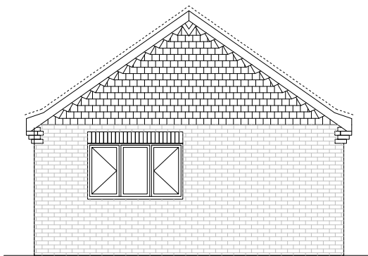
L/Side Elevation:
