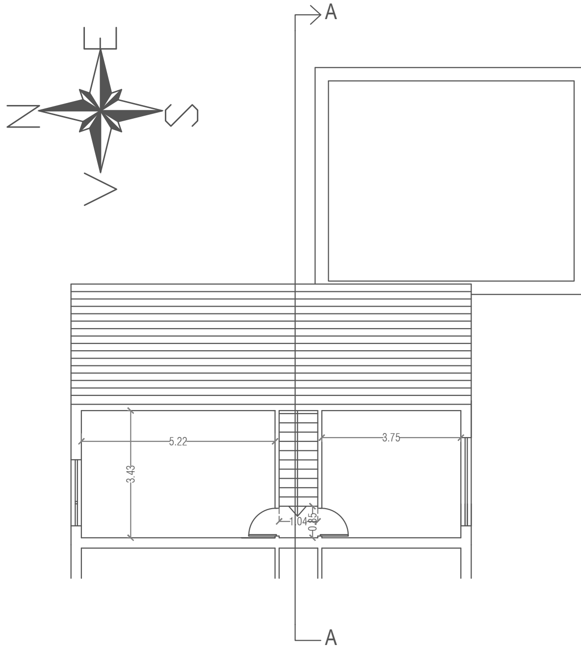
EXISTING FIRST FLOOR PLAN 1:100
