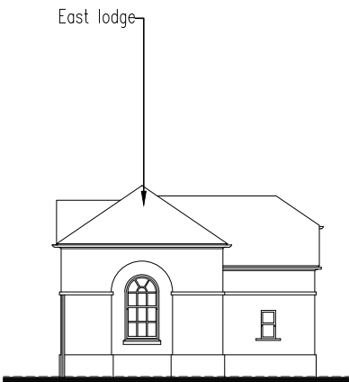
1:200 Existing South West Elevation
