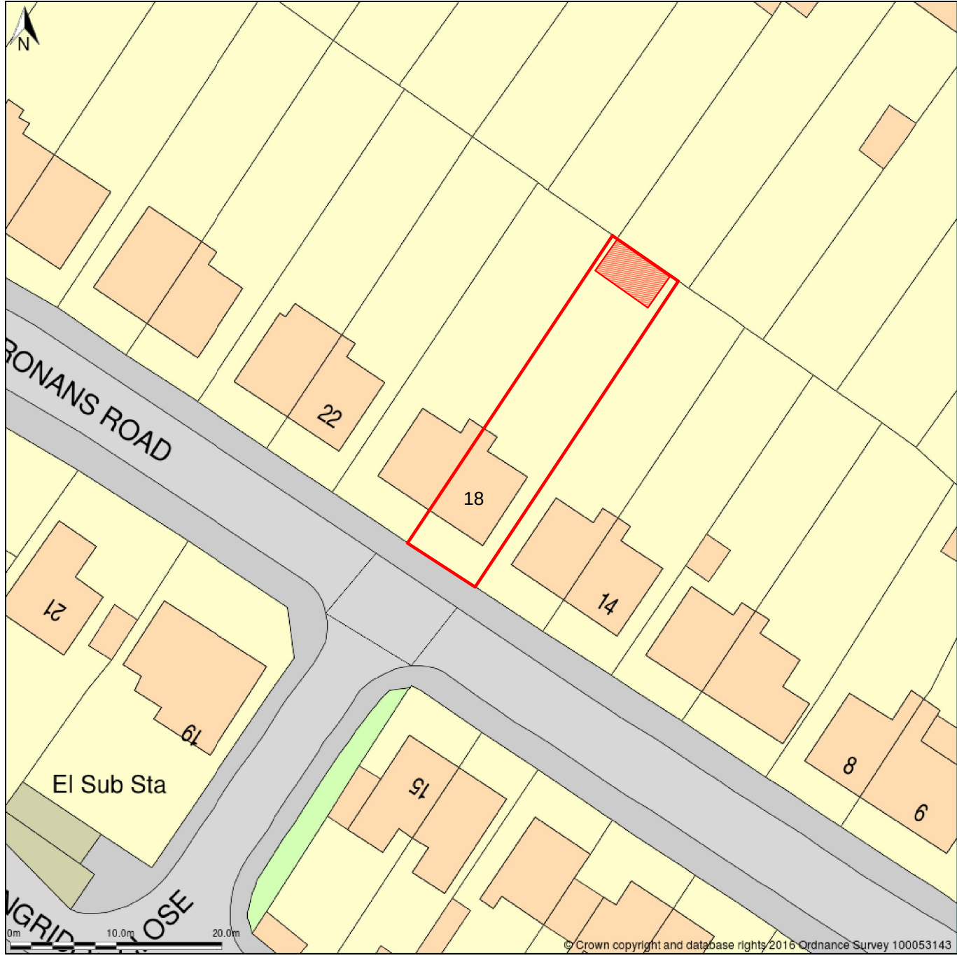
Block Plan 1:500
