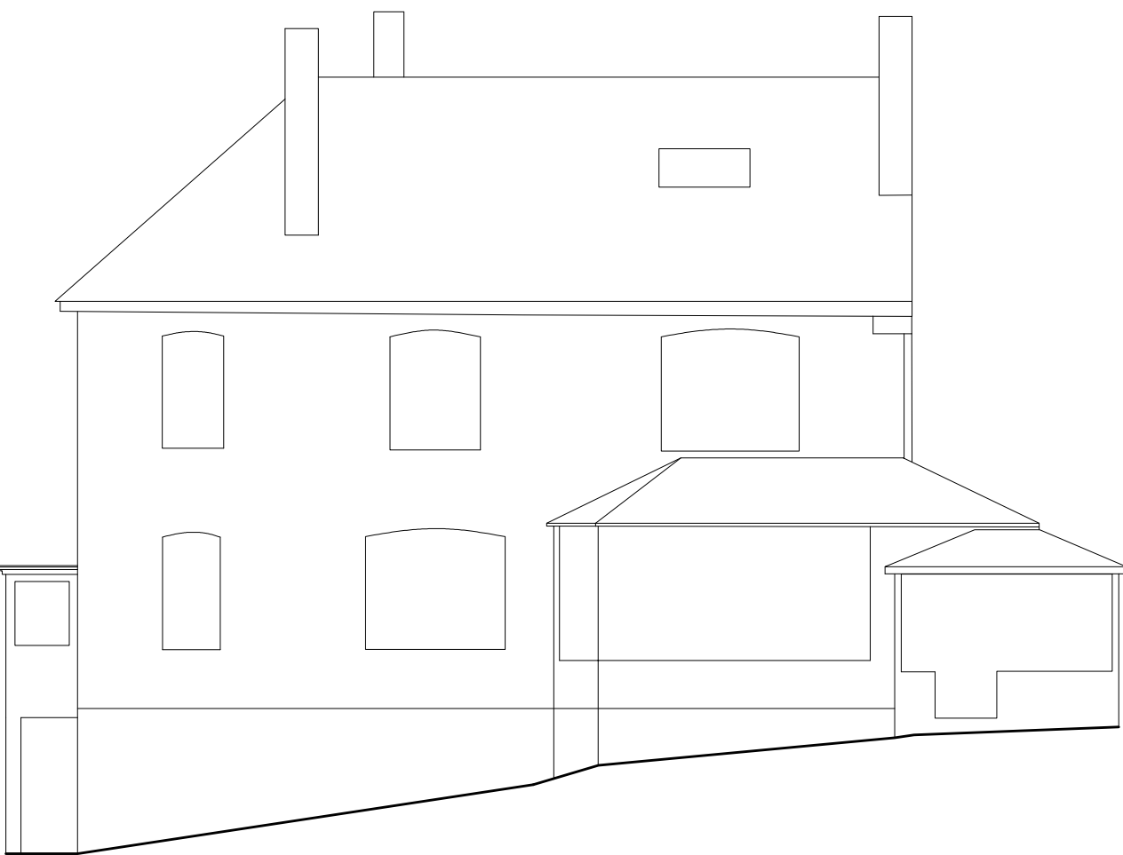
REAR ELEVATION
