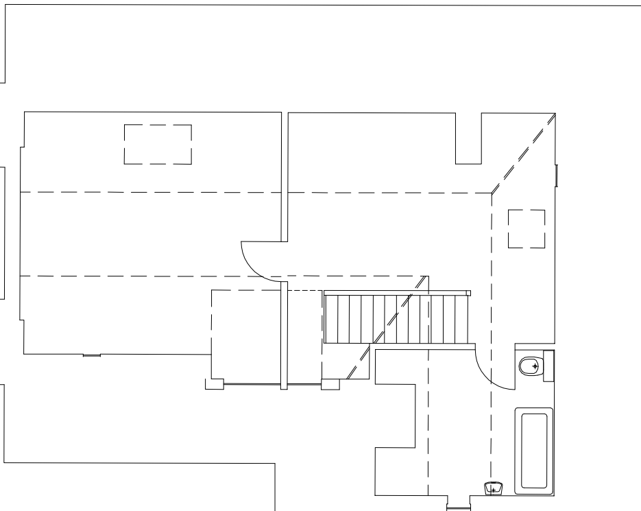
SECOND FLOOR
