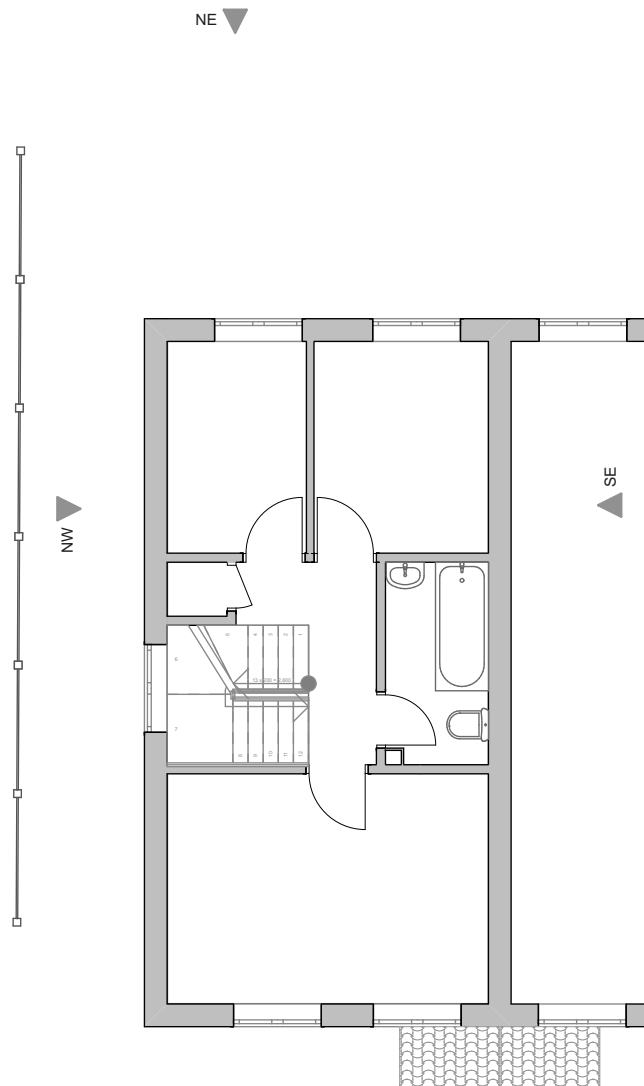
01-First Floor as existing 1:100
