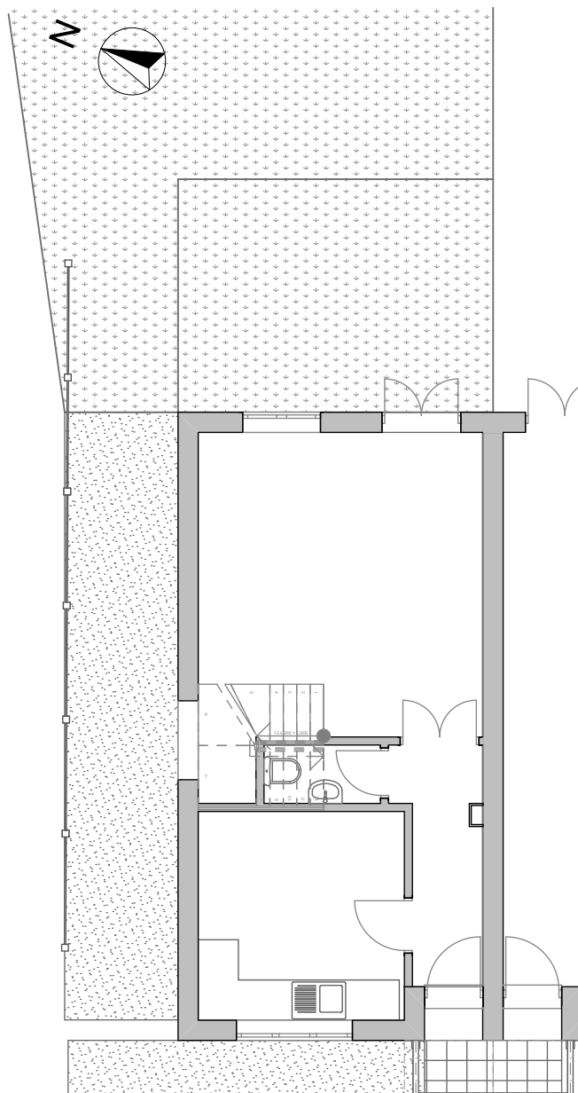
GF-Ground Floor as Existing 1:100
