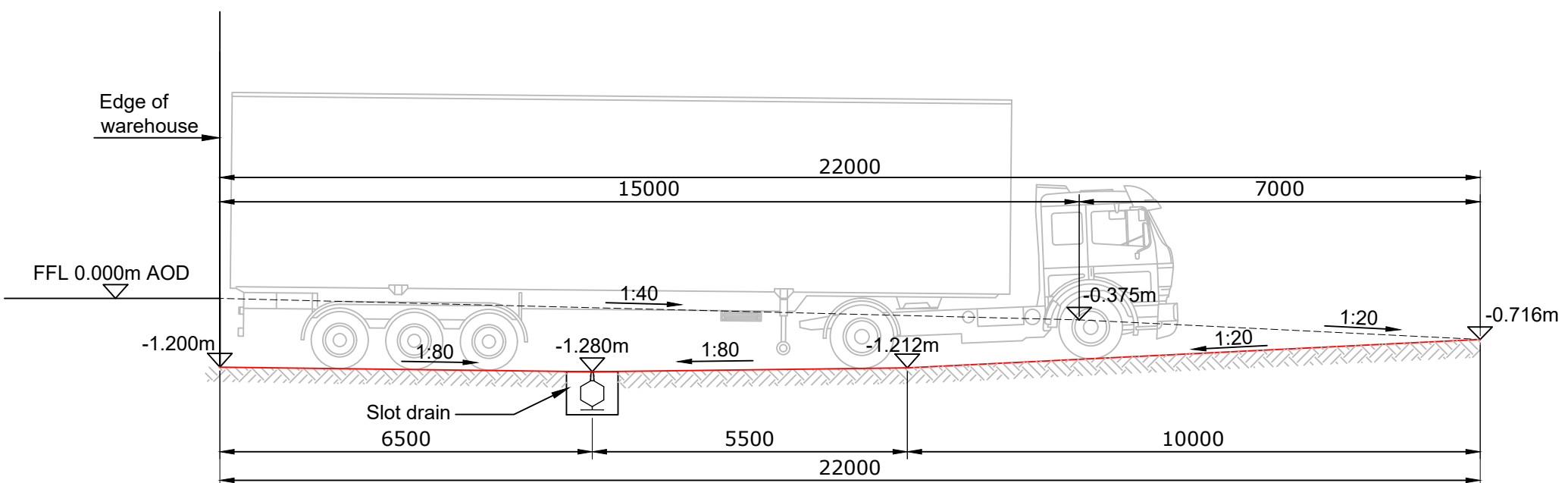
Section A-A - Typical Section Through Dock Levellers Scale 1:100
