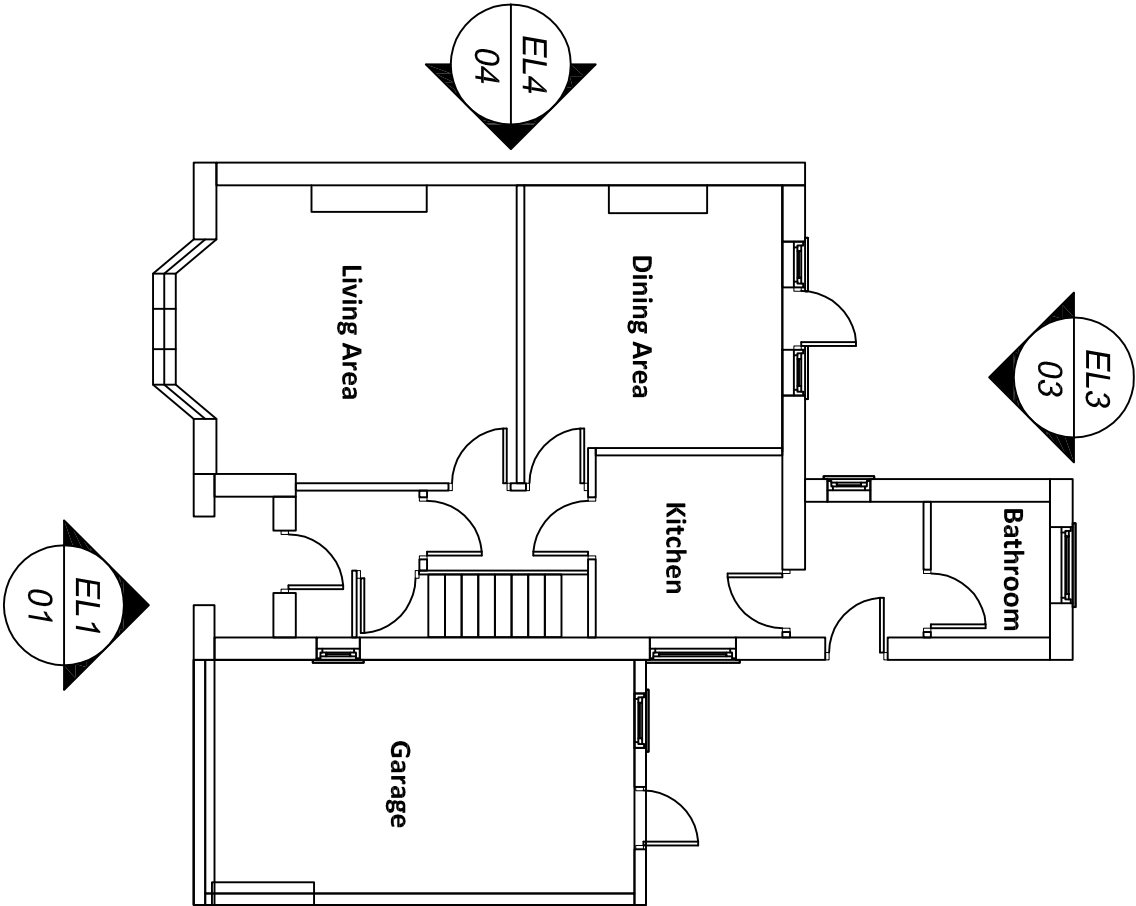
Existing Ground Floor Scale 1:100
