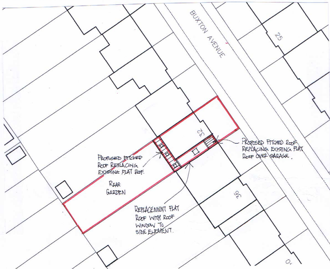
1-500 Scale Site Block Plan
