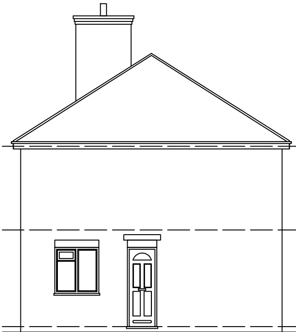
EXISTING SIDE-1 ELEVATION
