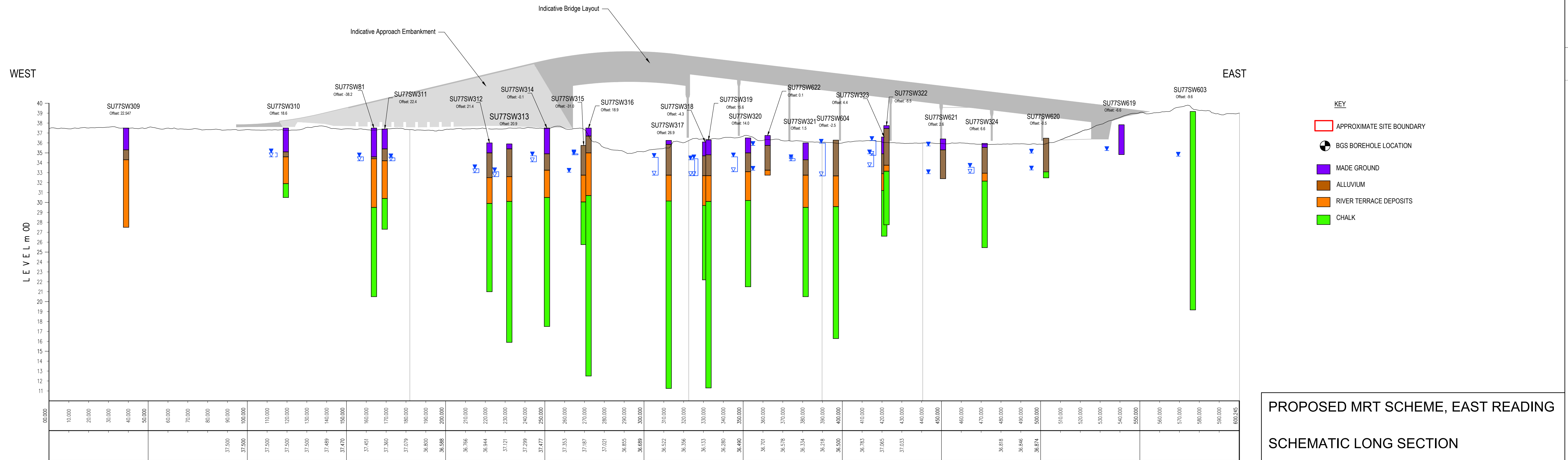
SCHEMATIC LONG SECTION Horizontal Scale 1:1000 - Vertical Scale 1:200
