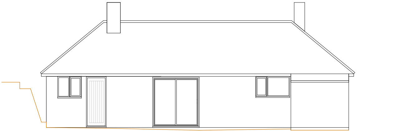
REAR ELEVATION
