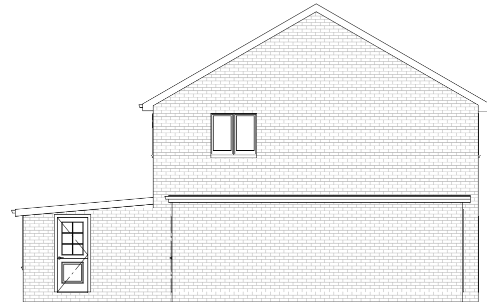
Proposed Right Elevation 1:100 @ A3
