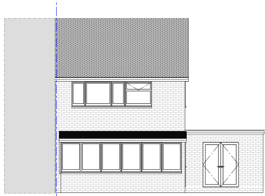
Proposed Rear Elevation 1:100 @ A3
