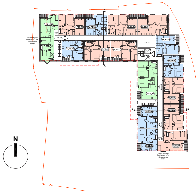
Typical/ 1st to 3rd Floor Plan (NTS): showing proposal compared with the footprint of the approved C2 scheme in red dashed line
