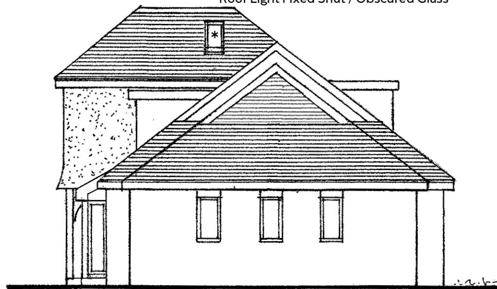
North Elevation
