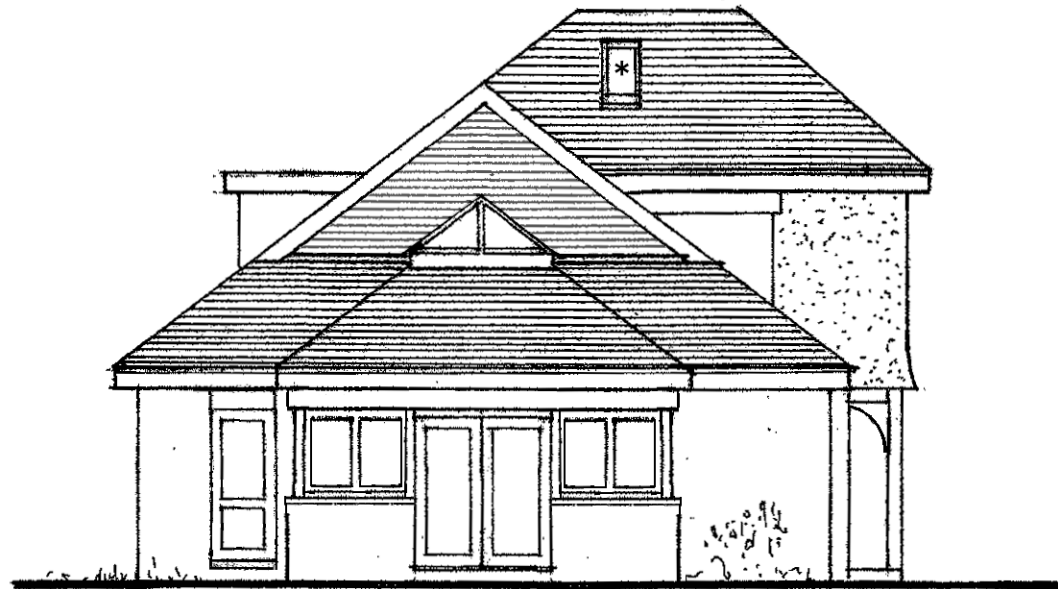
South Elevation
