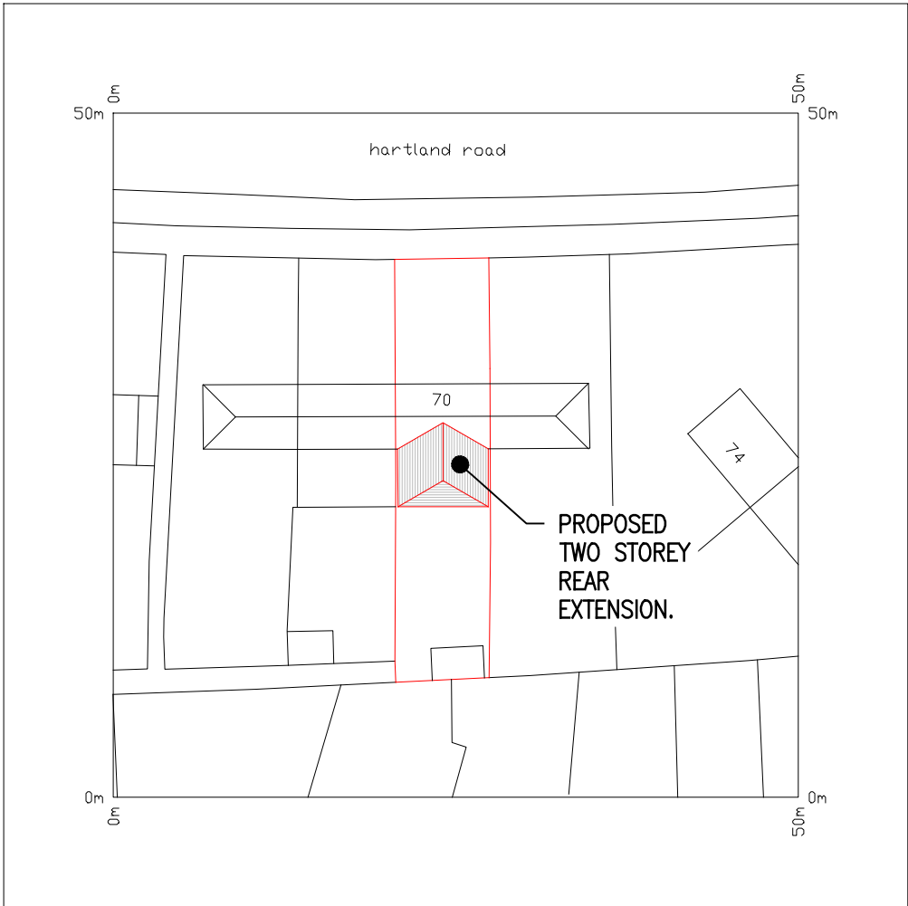
LOCATION PLAN 1:1250
