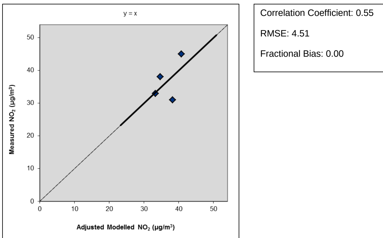
Figure 6: Comparison of Measured Total NO 2 to Final Adjusted Modelled Total NO 2 Concentrations.
