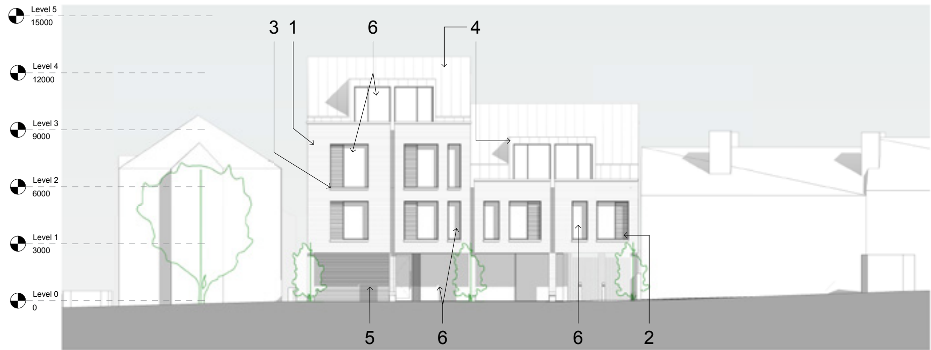
Silver Street Elevation 1 : 100
