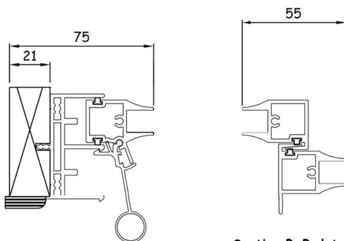
Section B-B detail Right Hand.
