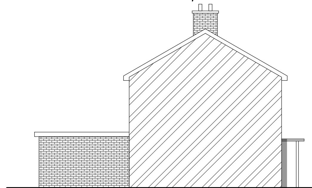
PROPOSED SIDE ELEVATION (FROM NO.33) SCALE 1/100
