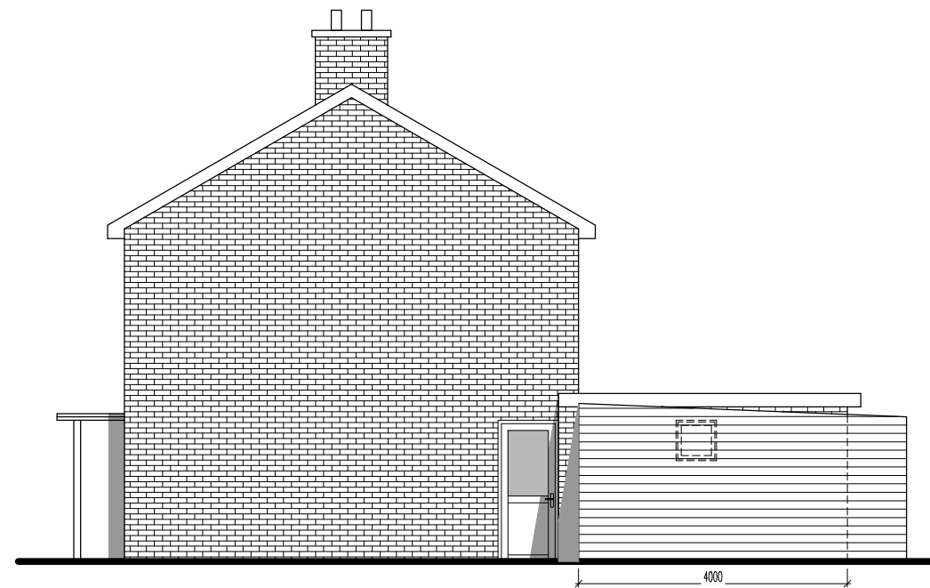
PROPOSED SIDE ELEVATION (FROM NO.37) SCALE 1/100
