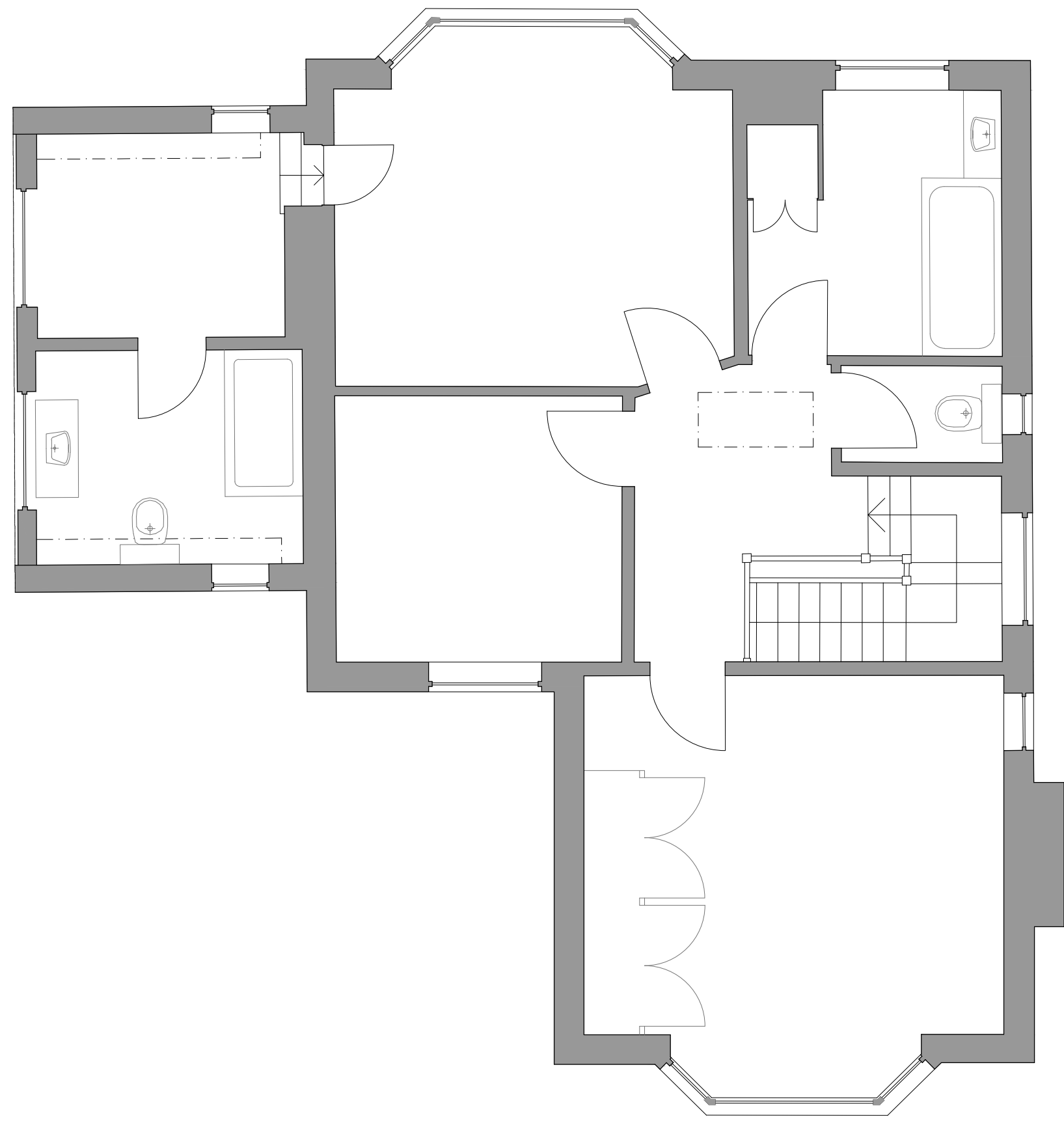
2 Existing First Floor Plan
