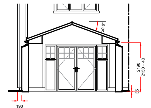
Rear Section
