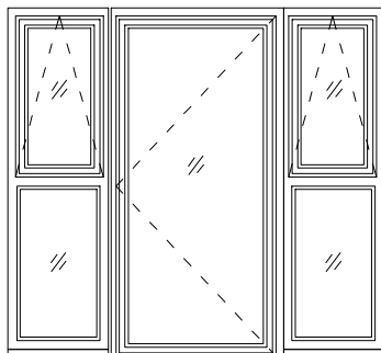
External Doors to Apartments White UPVC Doorsets - either Double Set of Single with Windows Either Side (see elevations for locations)
