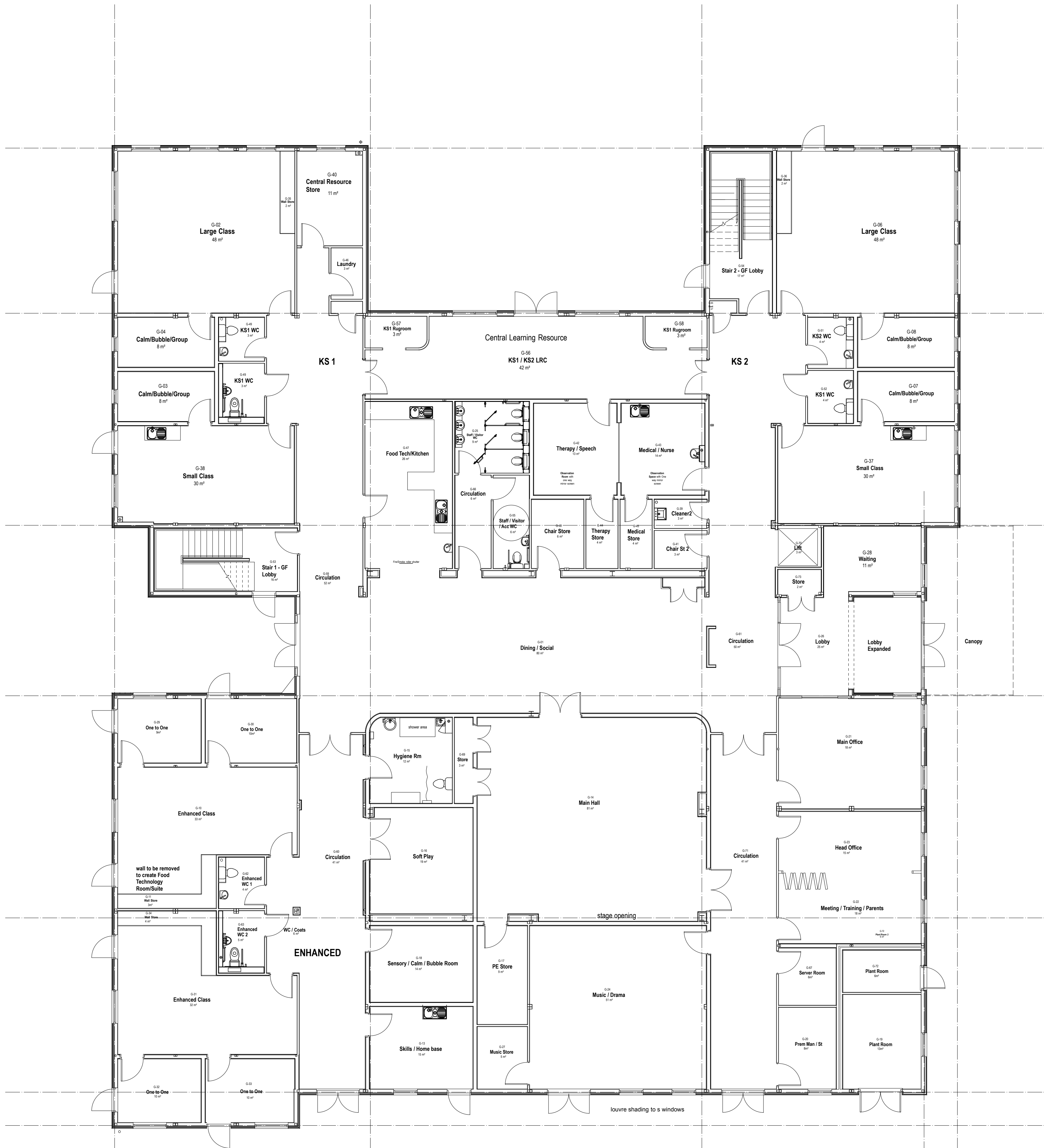
Ground Floor Layout (Proposed) 1 100 @A1 1 200 @A3
