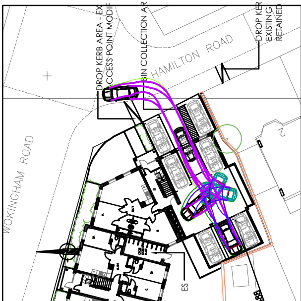
(4) LARGE SALOON CAR AUTOTRACK SWEEP PATH— ENTER SITE & PARKING SPACE IN FORWARD GEAR, REVERSE OUT, TWO POINT TURN AND EXIT SITE IN FORWARD GEAR.
