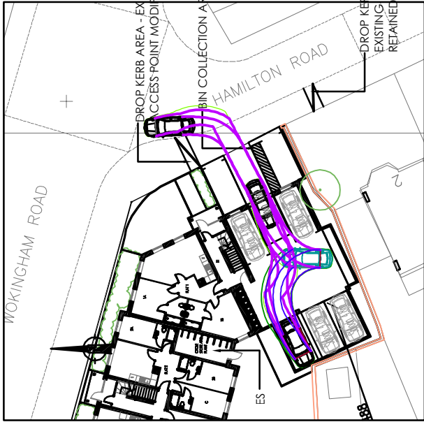
(5) LARGE SALOON CAR AUTOTRACK SWEEP PATH— ENTER SITE & PARKING SPACE IN FORWARD GEAR, REVERSE OUT AND EXIT SITE IN FORWARD GEAR.
