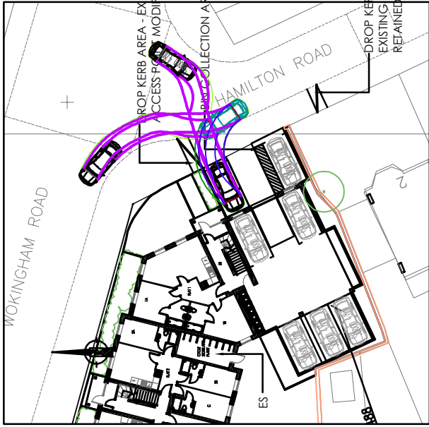
(1) LARGE SALOON CAR AUTOTRACK SWEEP PATH— ENTER PARKING SPACE IN FORWARD GEAR, REVERSE OUT AND TRAVEL TOWARDS WOKINGHAM ROAD IN FORWARD GEAR.
