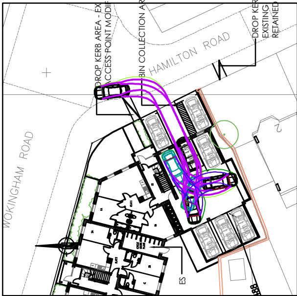
(7) LARGE SALOON CAR AUTOTRACK SWEEP PATH— ENTER SITE IN FORWARD GEAR, REVERSE INTO PARKING SPACE, EXIT SPACE & TWO POINT TURN AND EXIT SITE IN FORWARD GEAR.
