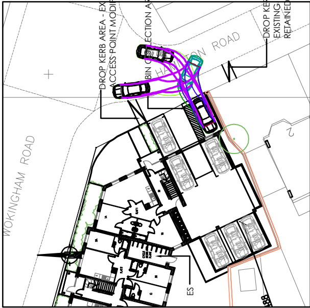
(2) LARGE SALOON CAR AUTOTRACK SWEEP PATH— ENTER PARKING SPACE IN FORWARD GEAR, REVERSE OUT AND TRAVEL TOWARDS WOKINGHAM ROAD IN FORWARD GEAR.
