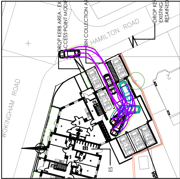
(6) LARGE SALOON CAR AUTOTRACK SWEEP PATH— ENTER SITE IN FORWARD GEAR, REVERSE INTO PARKING SPACE, EXIT SPACE & TWO POINT TURN AND EXIT SITE IN FORWARD GEAR.
