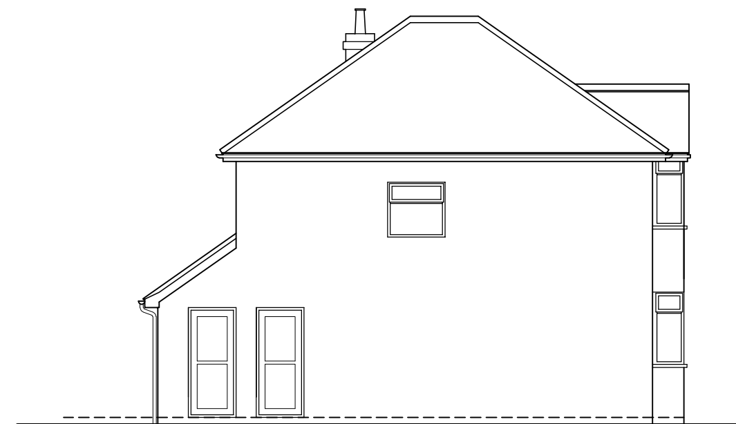
ORIGINAL SIDE ELEVATION
