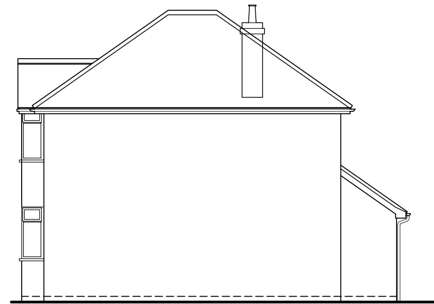
ORIGINAL SIDE ELEVATION
