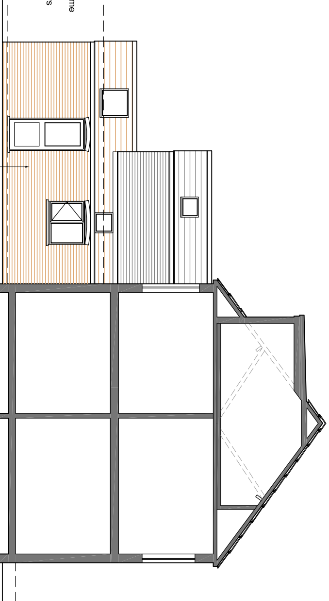
SECTION A-A & SIDE ELEVATION
