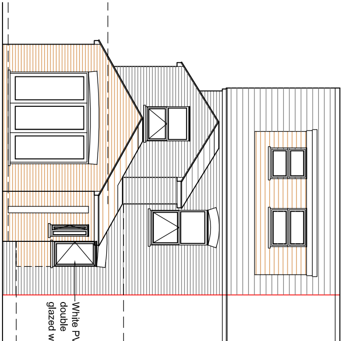
REAR ELEVATION
