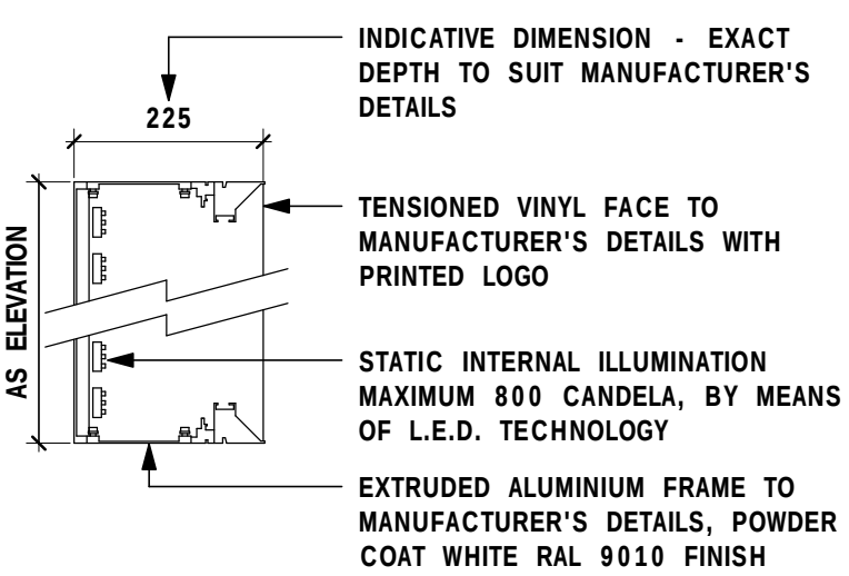
SECTION Z FLEX FACE SIGNAGE
