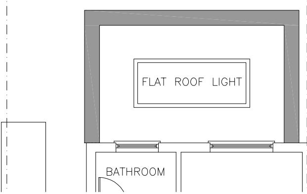
Roof Plan
