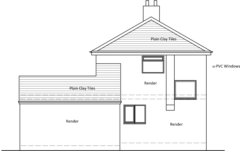
Extg Side Elevation
