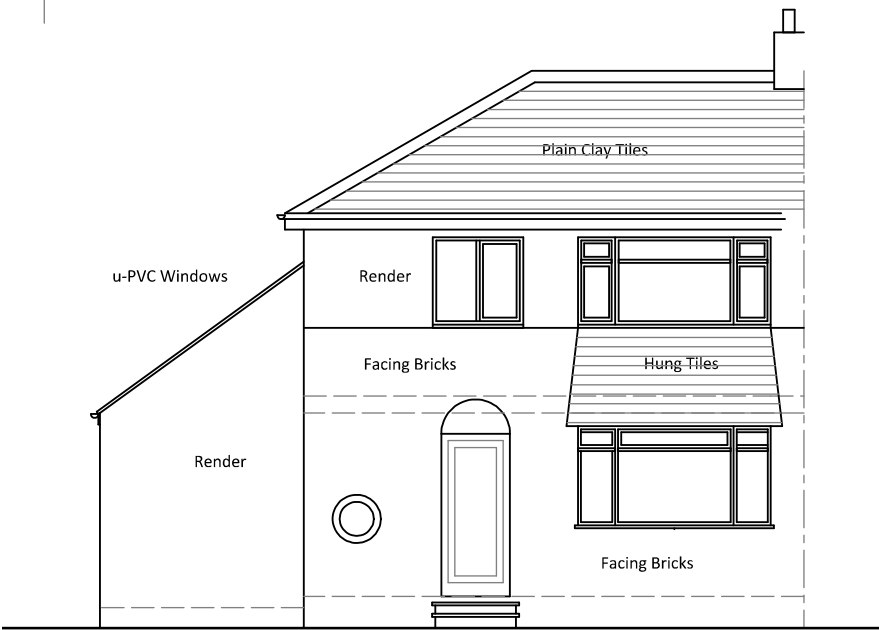
Extg Front Elevation
