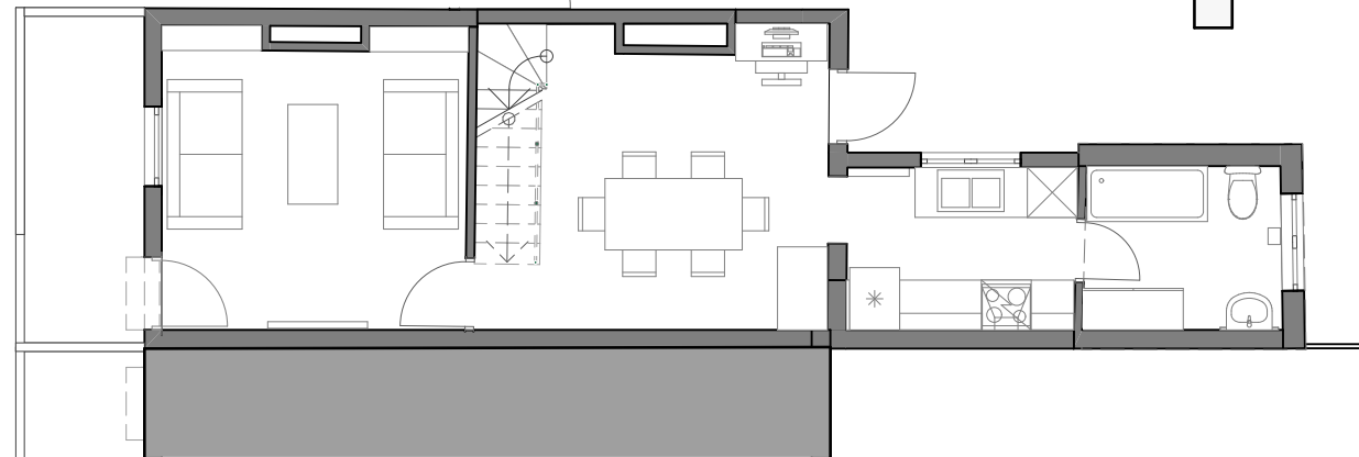
00 EXISTING GROUND FLOOR 1:100
