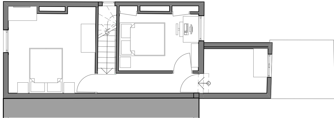
01 EXISTING FIRST FLOOR 1:100
