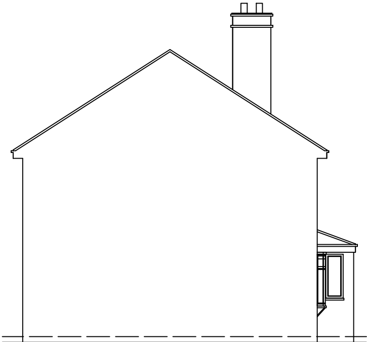
EXISTING SIDE-2 ELEVATION
